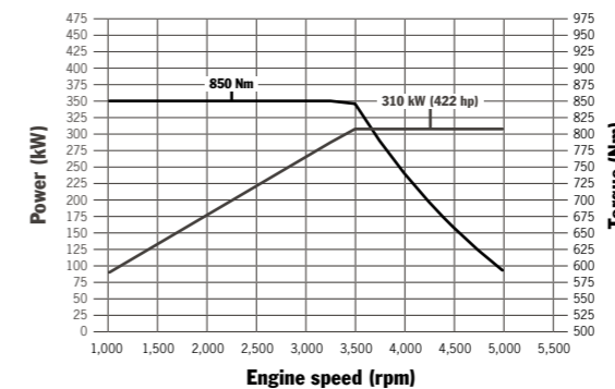
Panamera 4S Diesel: 310 kW (422 hp) between 3,500 and 5,000 rpm, 850 Nm between 1,000 and 3,250 rpm
